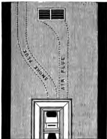
Fig. 10. —ELEVATION, SHOWING AIR AND SMOKE FLUES.
